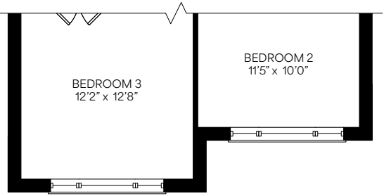
Second Floor Elevation D
